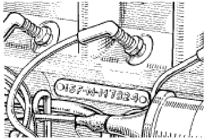
The Engine Number is stamped on a plate secured to the right-hand side of the cylinder block.
